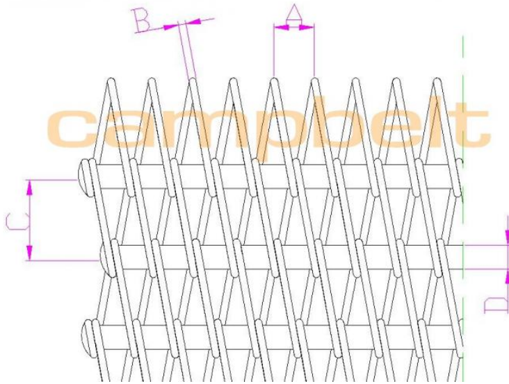
REINFORCED WEAVE CONVEYOR BELT (ARR)
